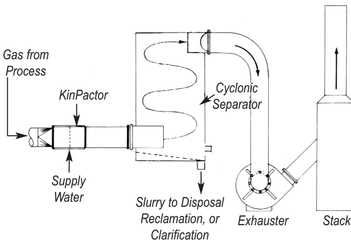
Figure 2. Typical Arrangement with Cyclonic Separator
