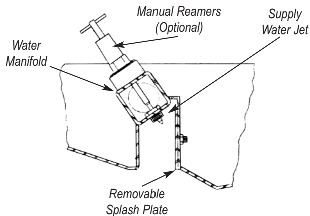
Figure 3. Detail H - Water Supply Assembly
