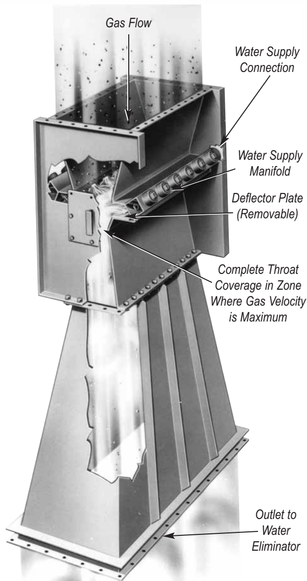
Figure 1. Cutaway View of the AAF KinPactor
